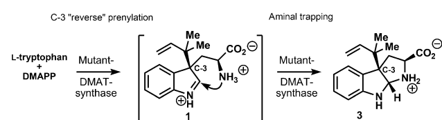
Scheme 1. The Arigoni and Wenkert biosynthetic hypothesis.
